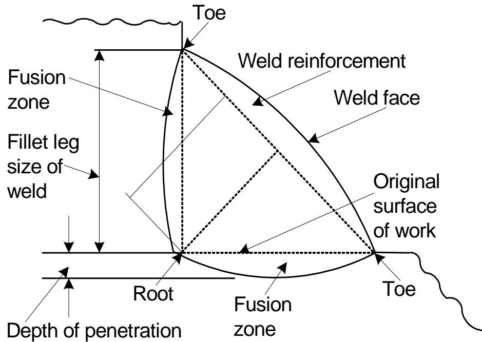
Figure 8.1.13 Fillet Weld Nomenclature
