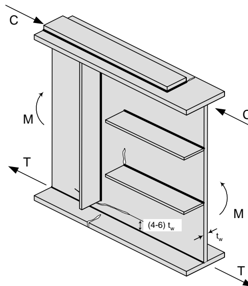
Figure 8.1.53 Cracks Perpendicular or Parallel to Applied Stress
